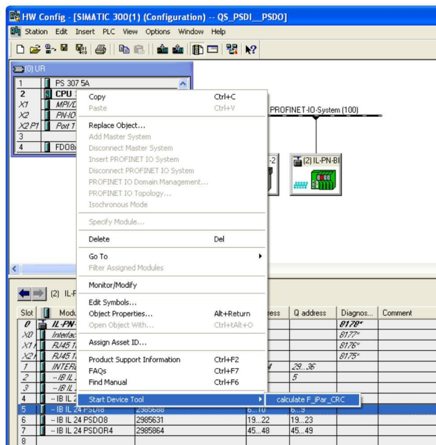
Figure 2-12 Starting the device tool
