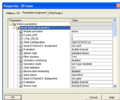
Figure 2-18 Channel parameterization
